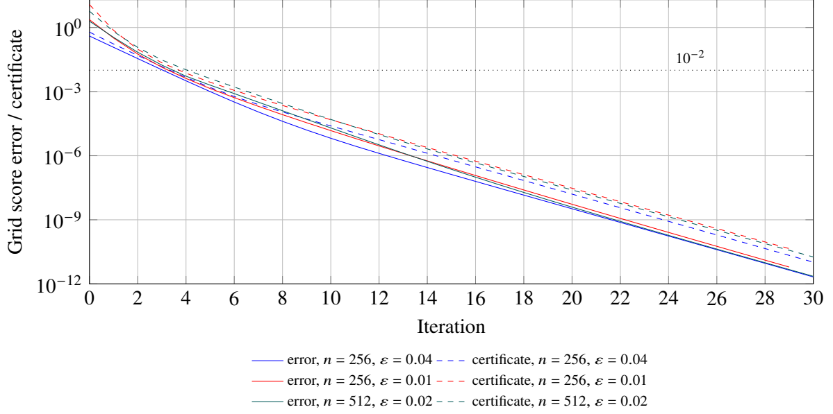
Figure 1: Grid score errors (solid) and a posteriori certificates (dashed) along actual symmetric self-Sinkhorn iterates. The plot is a numerical illustration; it does not establish the theorem.
